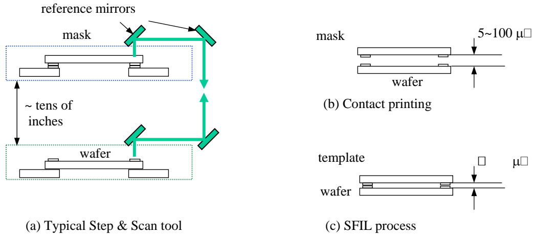
Figure 3. Mask (template) and wafer configurations for various lithography processes.
