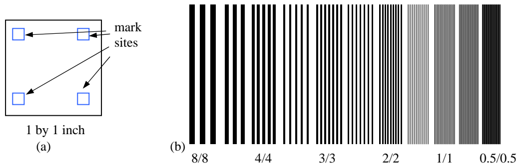
Figure 5. (a) Template with four sites of overlay marks. (b) Grating patterns with various line/space. Gratings are aligned in both X and Y directions.
